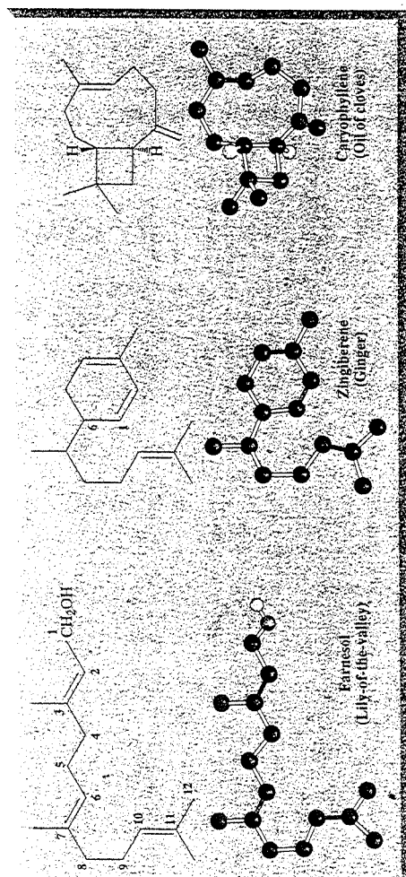
Figure 5.4 Three terpenes containing three isoprene units.
